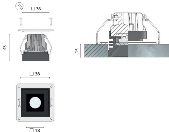
Power LED
