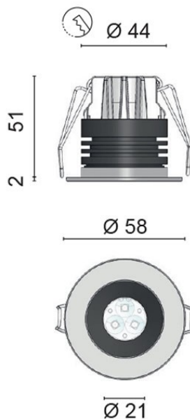
Power LED
